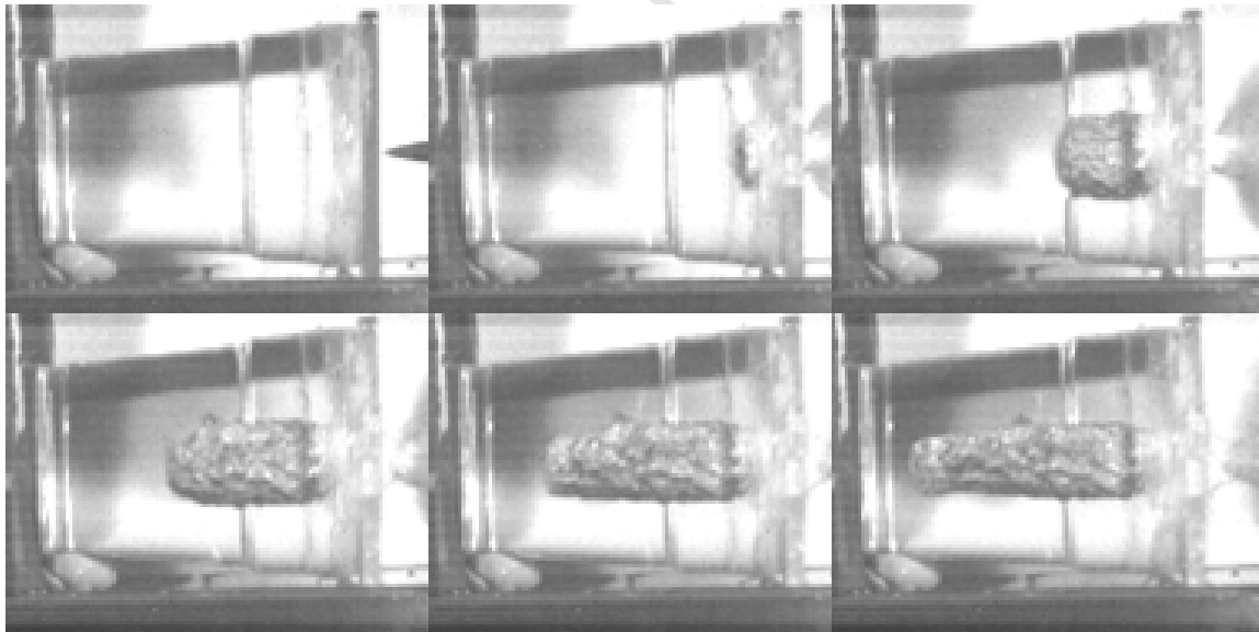
Figure 7: Penetration of a 7.62 mm × 51 mm NATO Ball round into a 6-mm glass-faced PRR target (beer-cup surround); time between frames = 50 μs. The curved surfaces of the beer-cup produce a lens effect and consequently the penetrating mass appears larger in diameter than it actually is.
