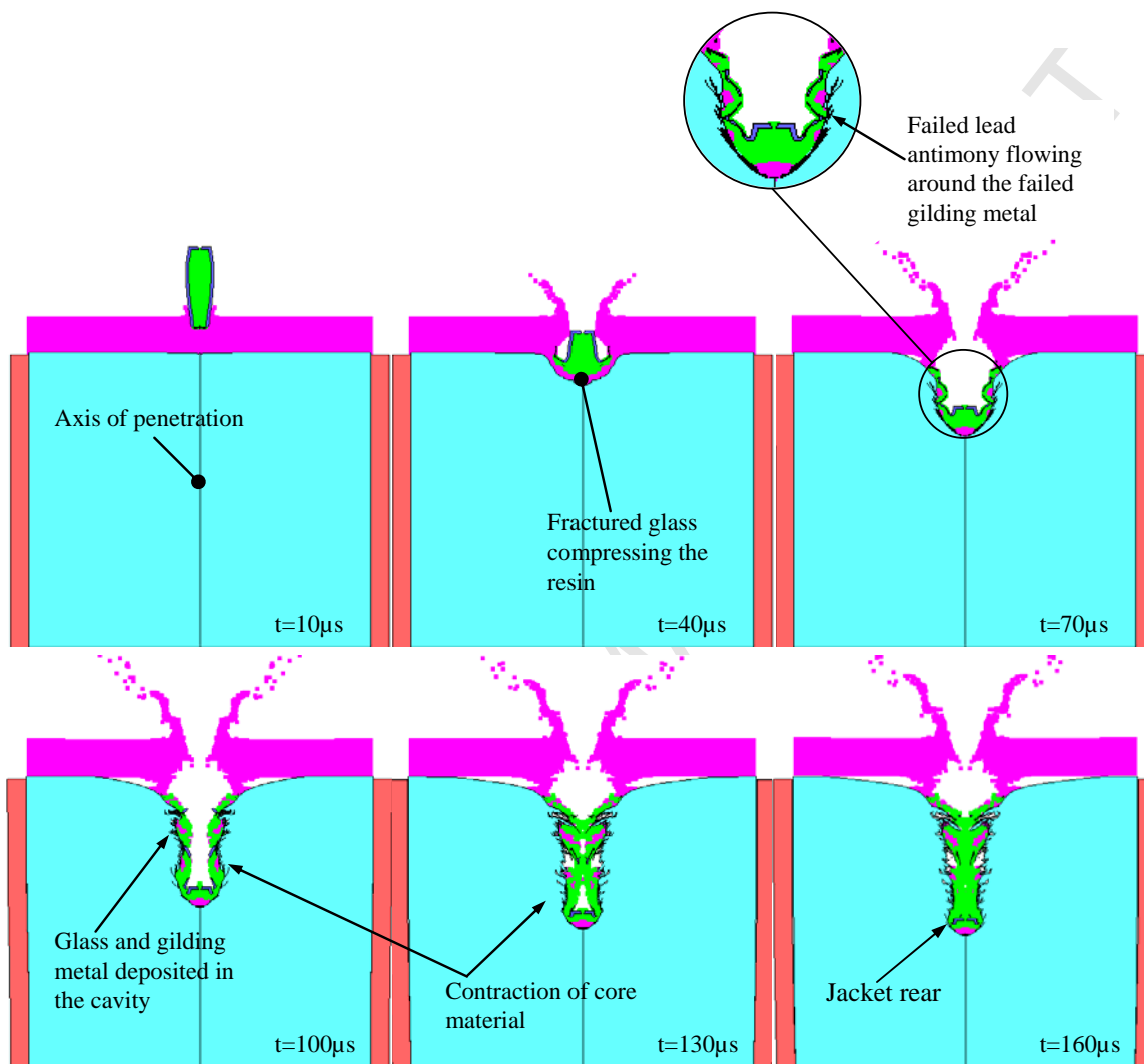
Figure 8: Numerical simulation of the penetration into a 10-mm glass-faced resin target with a polycarbonate surround; t = time from impact of glass face.
