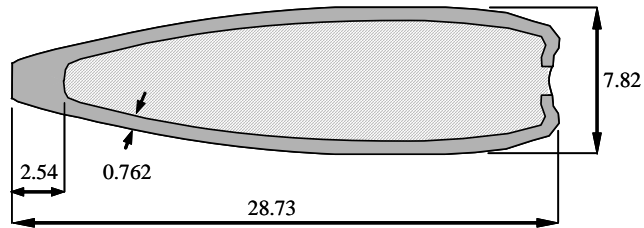
Figure 1: Geometry and key dimensions of the 7.62 mm \times 51 mm NATO ball bullet (dimensions in mm).
