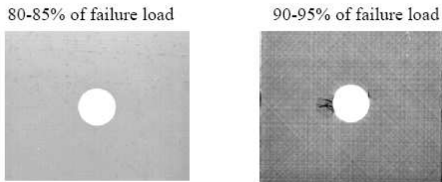
Fig. 9b) Damage development in a sublaminates-level scaled laminate [45/90/-45/0]_{4s} . Average failure load: 47.5 kN, hole diameter = 6.35mm.
