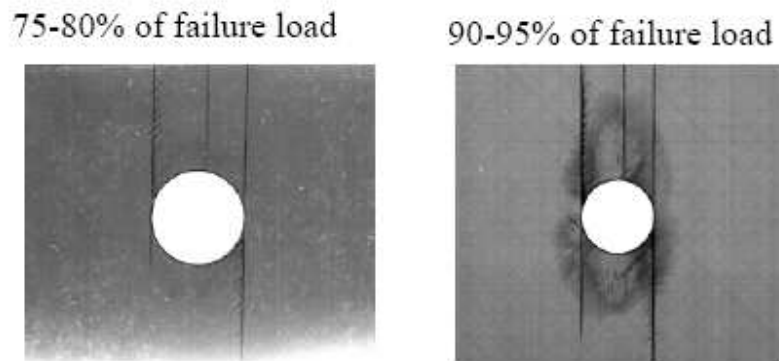
Fig. 9a) Damage development in a ply-level scaled laminate [45_4/90_4/-45_4/0_4]_s . Average failure load: 54.3 kN, hole diameter = 6.35mm. 47.5kN, Hole diameter = 6.35mm - [45/90/-45/0]_{4s}
