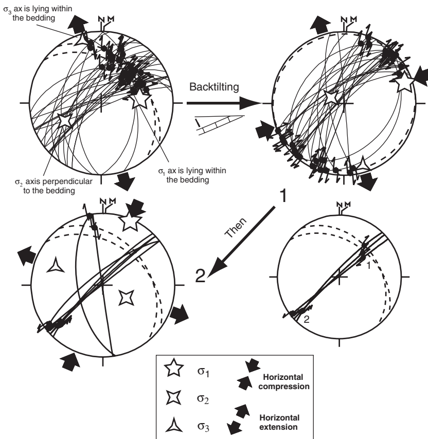
Fig. 10. Example of chronological relationships between faulting related to ENE–WSW compression and faulting related to N020° compression in limestones from the Champeh Member of the Gachsaran Fm. Stereodiagrams in the left part of the figure show striated microfaults in their current attitude (tilted strata), in contrast to the upper right diagram, in which faults related to ENE–WSW compression have been backtilted with bedding. The first strike-slip system predates folding as revealed by the attitude of principal stress axes and striations with respect to bedding; the N020° compression reactivates some faults consistent with the former stress regime and post-dates folding.
