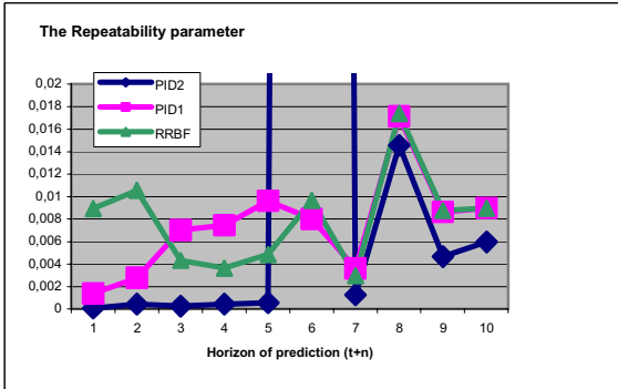
Fig. 16. Repeatability results obtained on Lorenz data set
