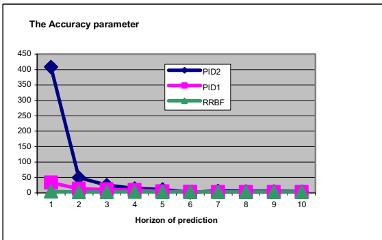
Fig. 17. Accuracy results obtained on Lorenz data set
