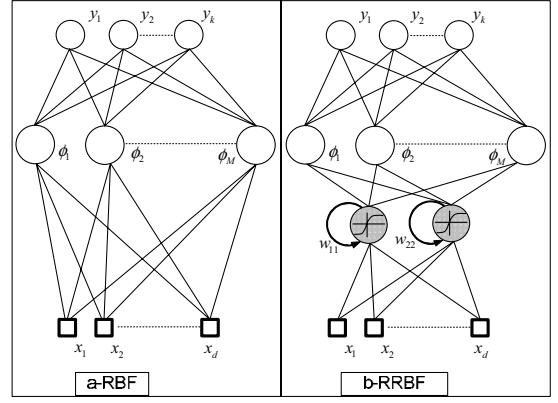
Fig. 5. Radial Basis Function and Recurrent Radial Basis Function networks
