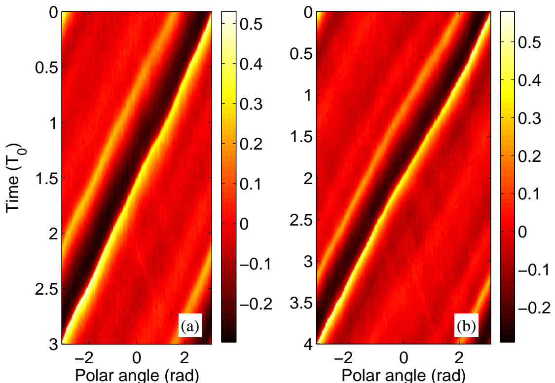
FIG. 5. (Color online) Pressure amplitude (gray scale in MPa) measured at z = 600 \text{ mm} for transient vortices of pitch 3 T_0 (subplot (a)) and 4 T_0 (subplot (b)) on a ring of width 0.5 \text{ mm} and radius 12 \text{ mm} and 15 \text{ mm} respectively. The vortices are made of 10 turns, but one located in the middle is presented
