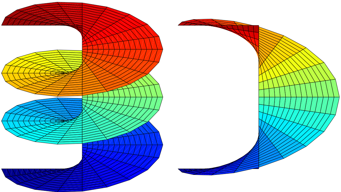
FIG. 1. (Color online) Helicoidal surface of pitch equal to 1 and truncated after 3 turns (left side), and of pitch equal to 3 truncated after 1 turn (right side)
