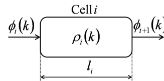
Fig. 2. Elementary cell.
