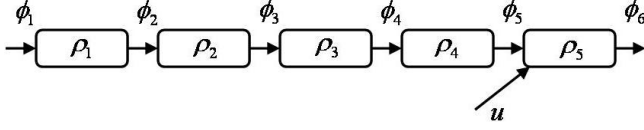
Fig. 5. On-ramp neighborhood.
