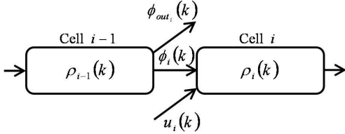
Fig. 3. Junction.
