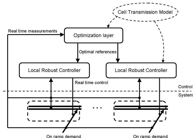
Fig. 1. Regulation scheme.
