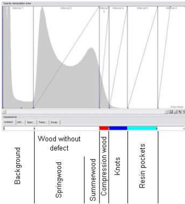
Figure 3 : Board grey level spectre
