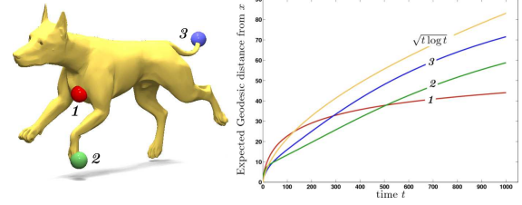
Figure 2: Expected geodesic distance \mathbb{E}(x, d(W_x^t)) between a point x and the Brownian motion W_x^t starting at x .
