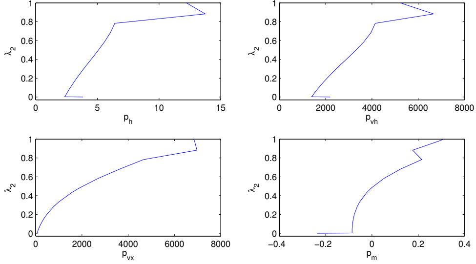
Figure 3: Evolution of the shooting function unknowns (p_h, p_{v_x}, p_{v_h}, p_m) (abscissa) with respect to homotopic parameter \lambda_2 (ordinate).
