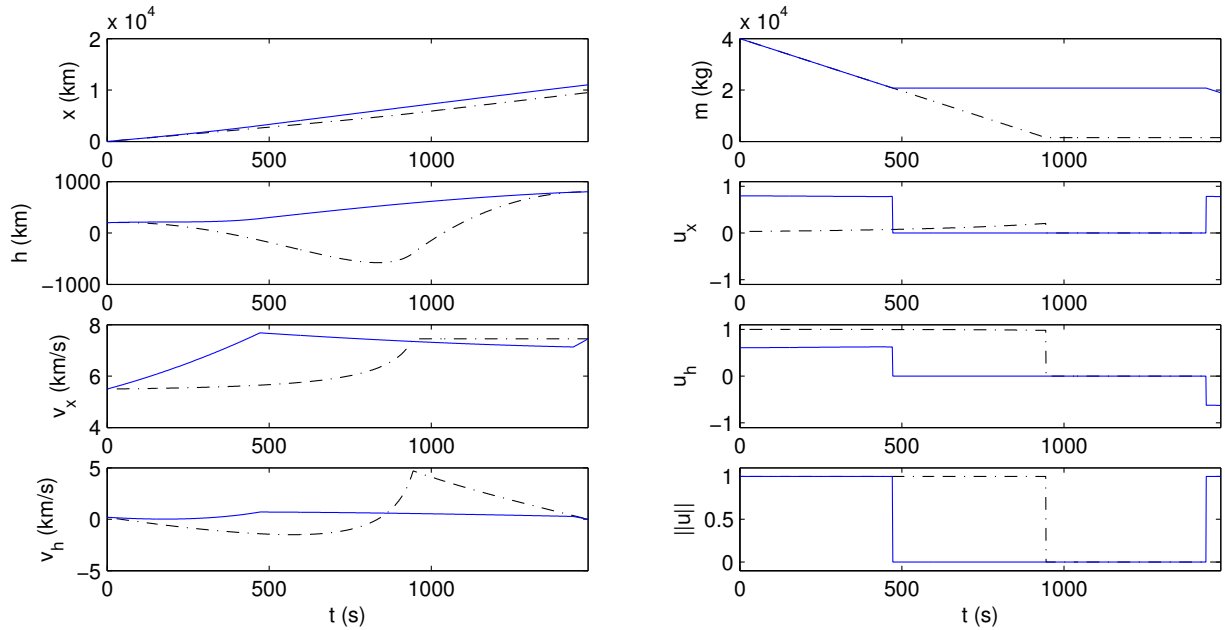
Figure 4: Trajectory and control strategy of (\mathbf{OCP})_{1,0} (dashed) and (\mathbf{OCP})_{1,1} (plain).
