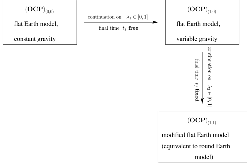
Figure 2: Continuation procedure
