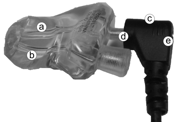
FIGURE 1 – Earplug with two inner bores; one to adjust the attenuation (b) and the other test bore (a) for insertion of the MIRE probe (c) with measurement (d) and reference (e) microphone. The measurement microphone measures the sound level in the ear canal behind the hearing protector whereas the reference microphone registers the incoming sound level.
