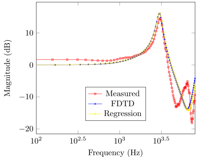
FIGURE 2 – Comparison of the transfer functions of one particular human ear as obtained by measurements (‘Measured’), FDTD simulations (‘FDTD’) and multiple linear regression (‘Regression’).
