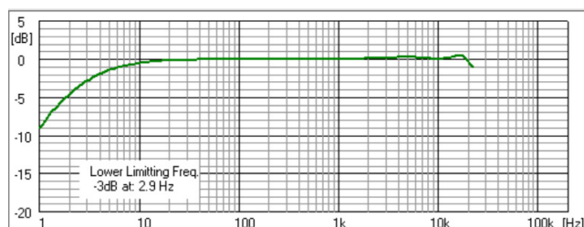
Fig. 1 Free – field microphone in free- field
