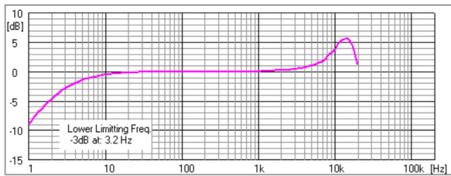
Fig. 4 Diffuse – field microphone in free – field
