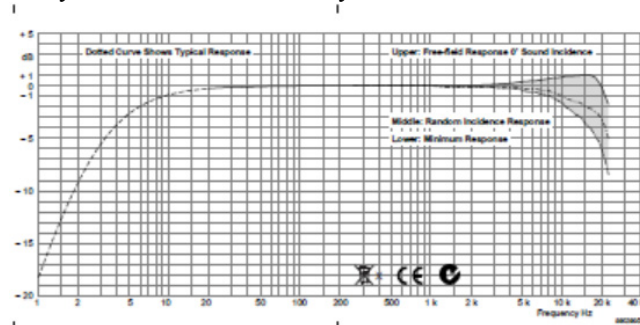
Fig. 7 Multi-field microphone calibration Chart
