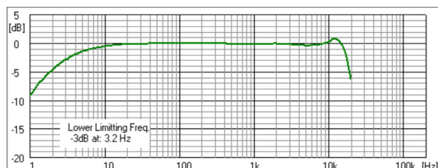
Fig. 3 Diffuse – field microphone in diffuse – field
