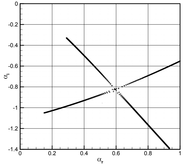
FIG. 7: Locus of spatial branches \alpha^+(L_\omega) and \alpha^-(L_\omega) as the L_\omega contour is lowered in the complex \omega - plane.
