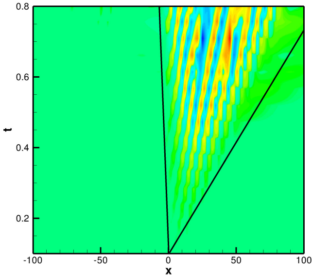
FIG. 6: Spatio-temporal evolution of v' at the center of the computational domain.
