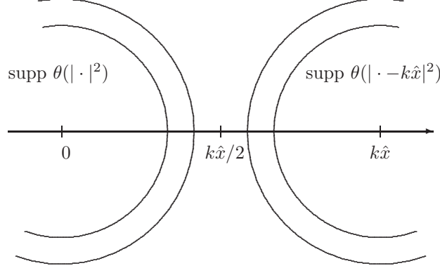
FIGURE 1. \text{supp } \theta \subset ]0, k^2/4[ .
