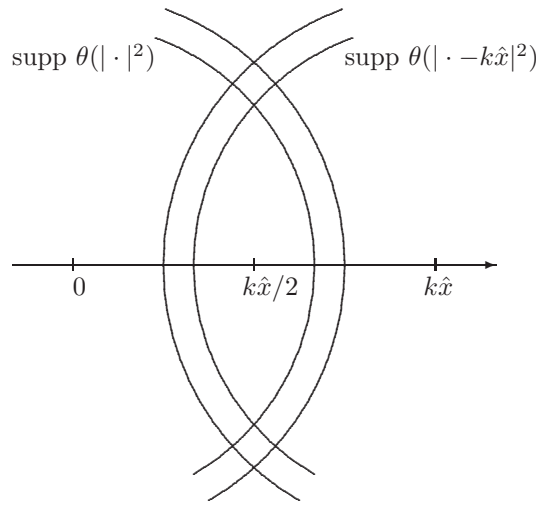
FIGURE 2. \text{supp } \theta \subset ]k^2/4, +\infty[ .
