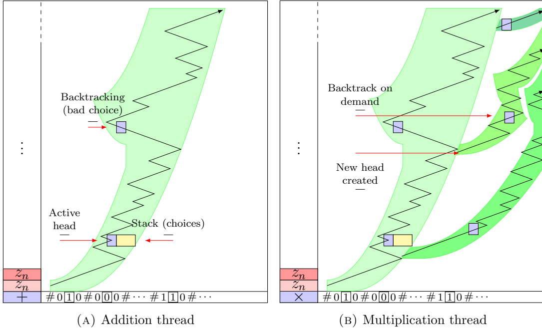
FIGURE 3. Computation threads
