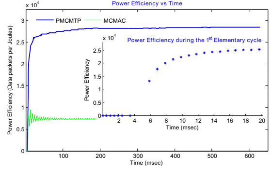
Fig. 14. Power Efficiency
