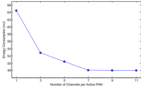
Fig. 8. Energy Consumption of the entire network vs Number of Channels
