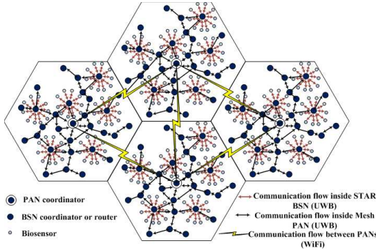
Fig. 1. WHSN architecture
