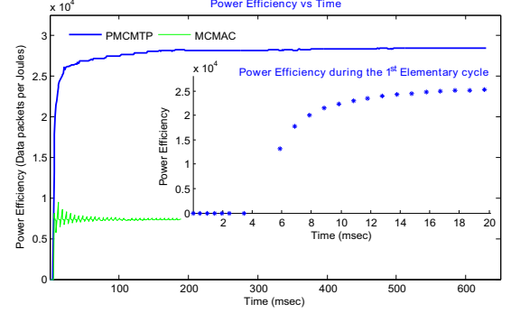
Fig. 14. Power Efficiency
