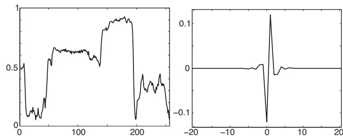
Fig. 2. Left: example of 1-D natural signal x_k used for the learning. Right: optimal filter \gamma^{(\infty)} learned by our method.
