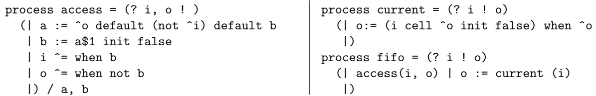
Figure 13. A one-place first-in first-out buffer in SIGNAL
