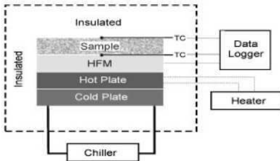
Figure 20: The measurement setup from de Darkwa et al. [71].
