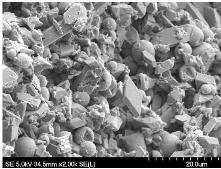
Figure 15: SEM photography of a concrete wall containing micro-encapsulated PCM, from Schossig and al. [61].
