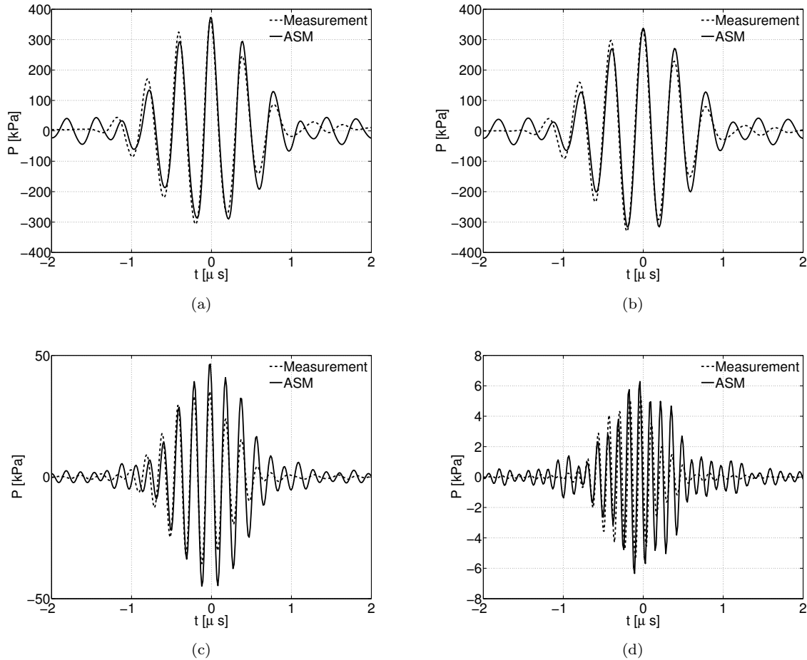
FIG. 3: Comparison between measurements and simulation. Full line presents ASM method results, while dashed line is the measurements. On Fig.3(a) is the acquired pulse, while on the Fig.3(b), Fig.3(c) and Fig.3(d) are the fundamental, second and third harmonic respectively. Note that there is some over estimation of the harmonics, while phase of each harmonic is good predicted. Also note that amplitude scale is not the same for all harmonics, meaning that assumption Eq. (26) is fully acceptable
