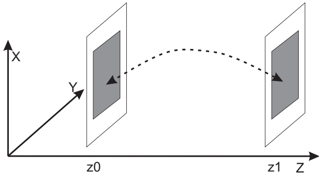
FIG. 1: Propagation of a plane from z_0 to z_1
