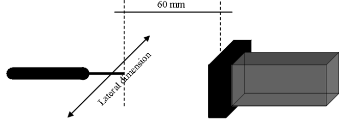
FIG. 2: Measurement setup. The hydrophone is placed in focal spot of the each transducer surface. Lateral profile was measured with a 3D xyz system
