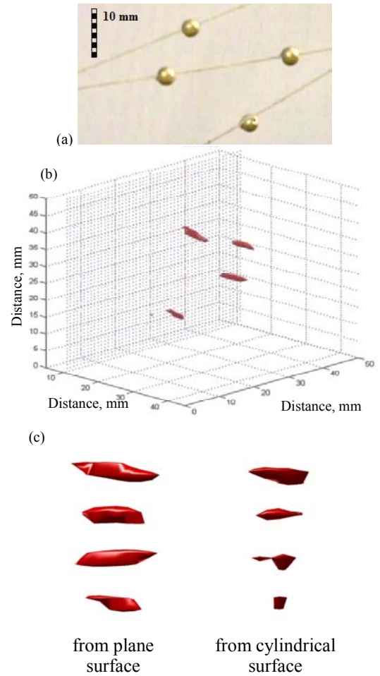
Figure 3. (a) Set of 3-mm diameter plastic beads; (b) isosurfaces with 0.8 level from maximum amplitude value calculated from the plane surface; (c) shape of the isosurfaces with 0.8 level from maximum amplitude value calculated from the plane (left) and cylindrical (right) surfaces.
