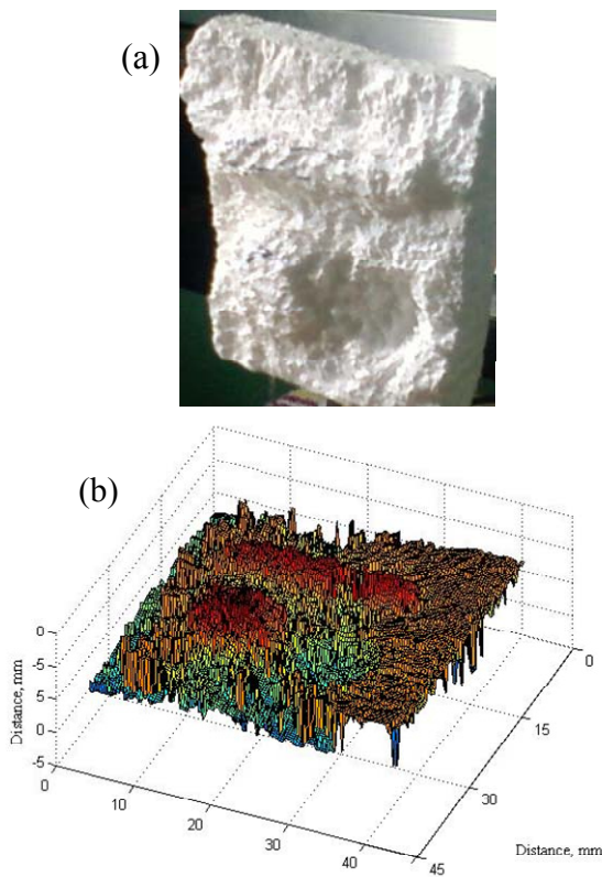
Figure 4. (a) Surface of Styrofoam sample. (b) Reconstructed surface of Styrofoam sample.
