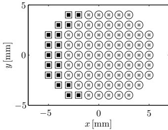
FIG. 3: Division of the contact area : quasi-static case, \eta = 10^{-3} . Stick zone : \circ (CONTACT), \times (interaction model) ; Slip zone : \square (CONTACT), \blacksquare , filled (interaction model).
