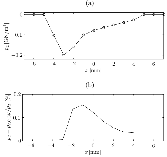
FIG. 5: Lateral tangential stress on line y = 0 : quasi-static case, \eta = 10^{-3} . (a) Amplitude : — interaction model, \circ CONTACT ; (b) relative difference.
