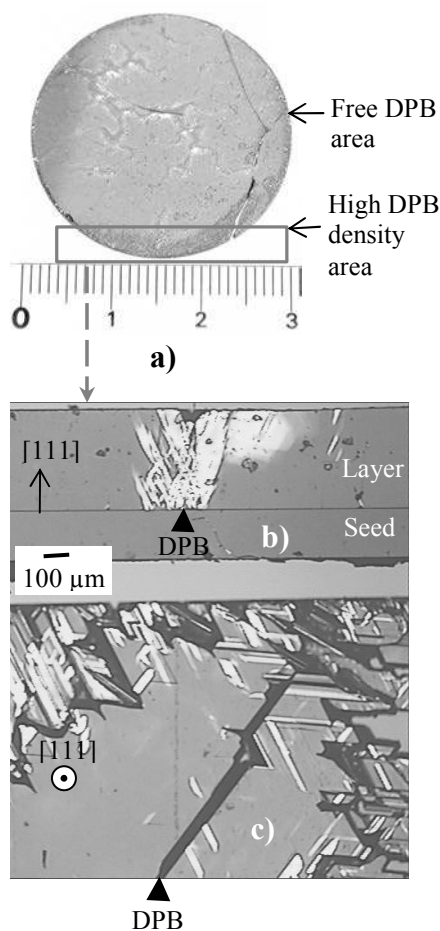
Fig. 1: a) 30 mm diameter 3C-SiC thick layer nearly free of DPB. Cross-polarized optical microscopy in the high DPB density area. DPBs are observed b) in cross-section and c) in planar view geometries.
