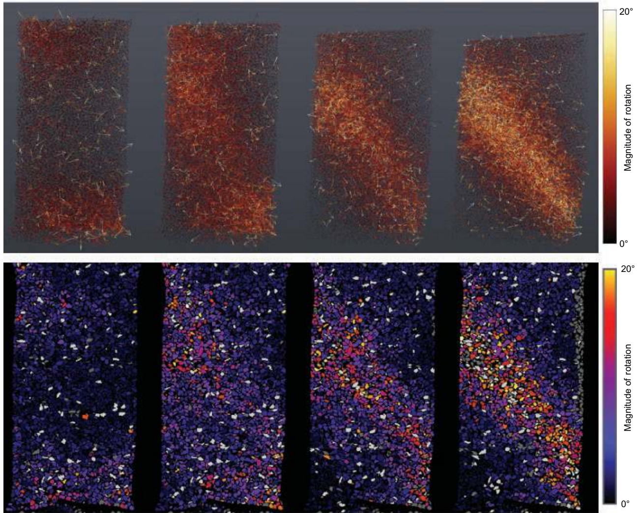
Fig 5. Discrete V-DIC derived incremental grain rotations for increments 3–4, 4–5, 5–6 and 6–7 (previous increments showed much the same picture as 3–4). Top: 3D volume view of the rotation vectors (axes of rotation for each grain are plotted with their length and colour indicating the magnitude of the rotation about these axes). Bottom: magnitude of the grain rotations plotted for vertical slices through the middle of the specimen at an equivalent position to Figs 2 and 3; note that the grains are plotted in the configuration at the start of the test for all increments. Grains coloured grey are those for which the image correlation was not successful and those coloured white are those with a rotation above a threshold value of 20^\circ (corresponding also to the long white vectors in the upper images)
