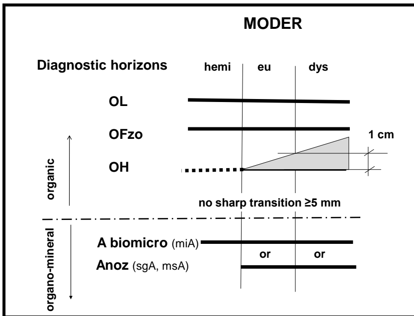
Fig. 10b. Terroforms, second level of classification of Amphi and Moder. Lines: diagnostic horizons, sequence as in real profile. Columns: second level of classification (example of Mull forms: eumull, mesomull, oligomull, dysmull).
