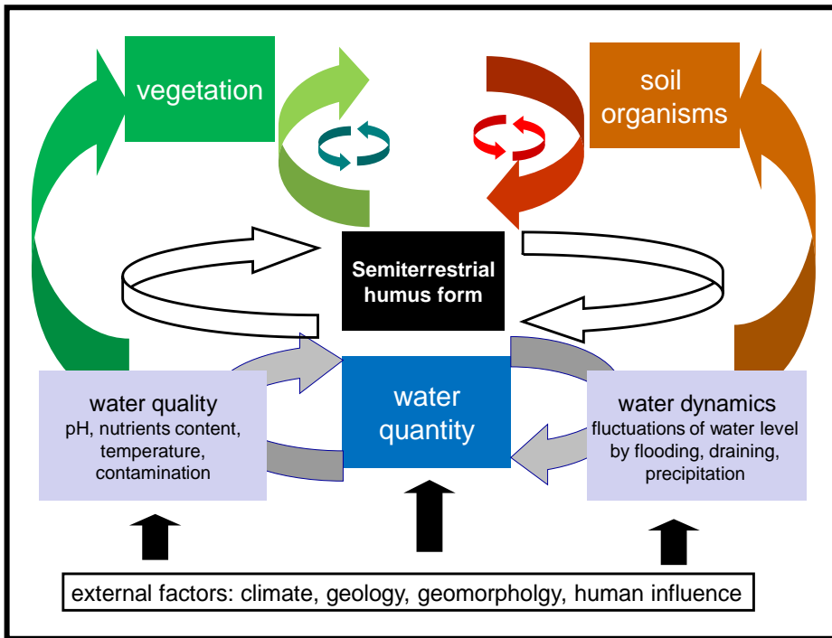
Fig. 24. Interacting ecological factors in semiterrestrial humus forms.
