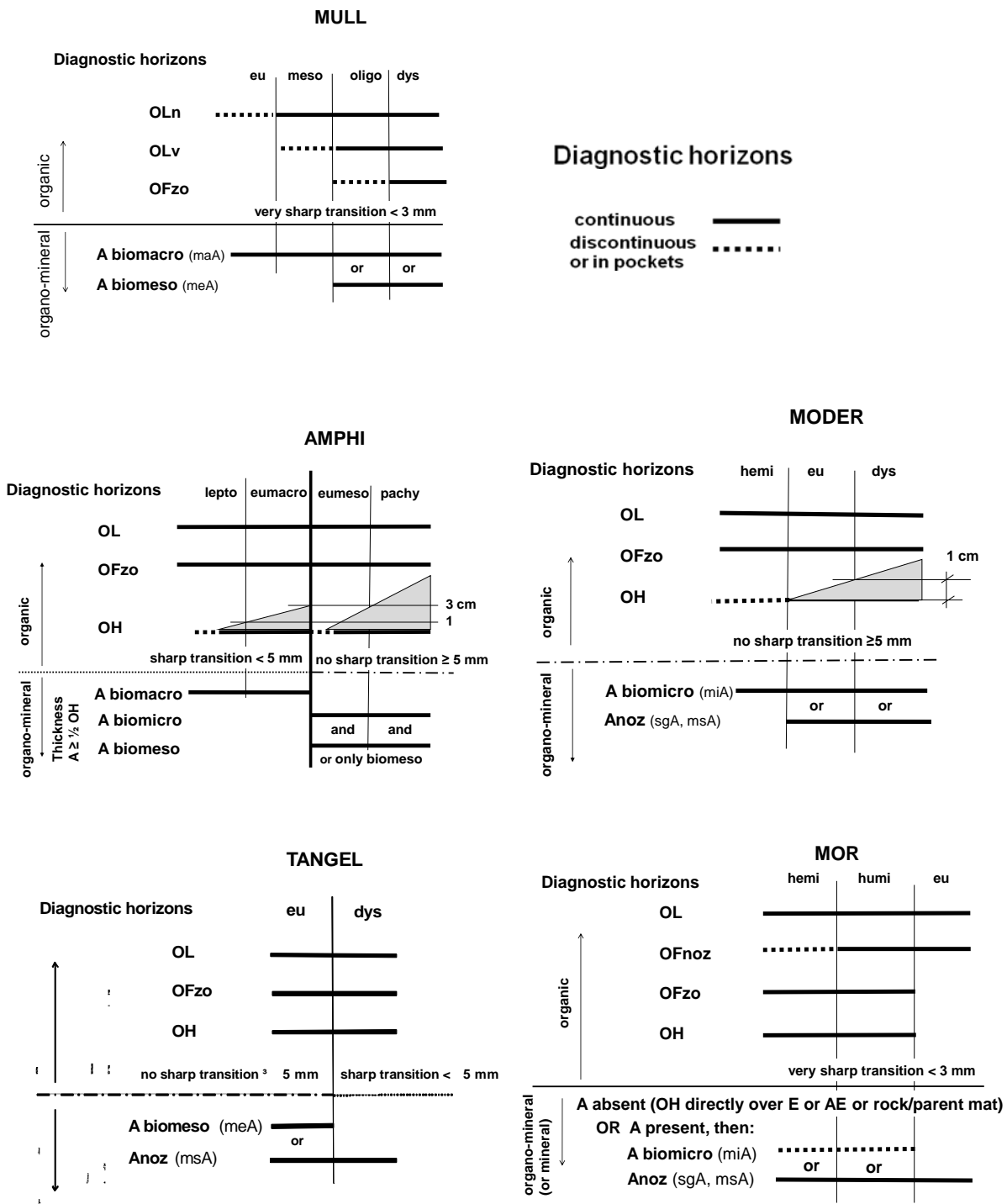
Fig. 10. Terroforms, second level of classification. Lines: diagnostic horizons, sequence as in real profile. Columns: second level of classification (example of Mull forms: eumull, mesomull, oligomull, dysmull).
