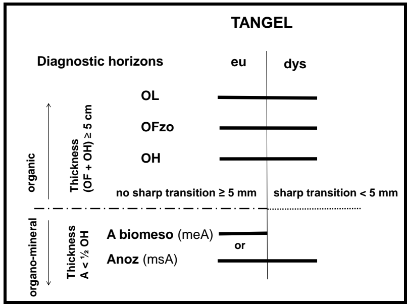
Fig. 10c. Terroforms, second level of classification of Mor and Tangel. Lines: diagnostic horizons, sequence as in real profile. Columns: second level of classification (example of Mull forms: eumull, mesomull, oligomull, dysmull).
