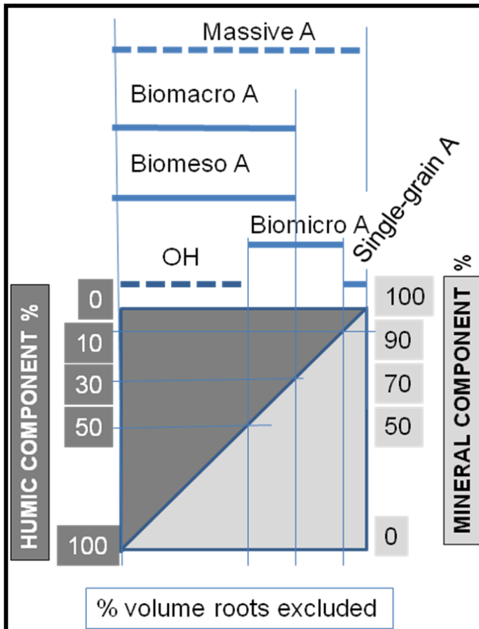
Fig. 8. Range of the ratio of humic and mineral component in the different A horizons, distinguished by the naked eye or with the help of a 5-10 X magnifying hand lens. At this scale, mineral grains included in animal droppings are considered as humic component; only free or very weakly bound grains are considered as mineral component. Biomacro- and biomesostrucures differ by the mean size of the peds but not by the HC/MC ratio, which is generally very high (often 100%). On the right side, the biomicrostructured A becomes single grain A when MC rises to more than 90% of the horizon volume; on the left side, biomicrostructured A becomes OH horizon when MC decreases until less than 50% of the horizon volume. The massive structure is independent of the HC/MC ratio.
