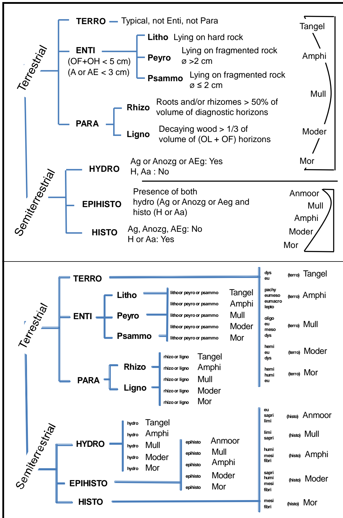
Fig. 2. The European tree of humus form classification. The most important level of classification is defined in the field, detecting the morpho-functional result (the sequence of diagnostic horizons) of specific biological activities. Considering the transitional group of Hydroforms separately, five Terrestrial biological types (Tangel, Amphi, Mull, Moder, Mor) and five Semiterrestrial ones (Mor, Moder, Amphi, Mull, Anmoor) may rank along a gradient of increasing then decreasing biological activity within each group of humus forms.
