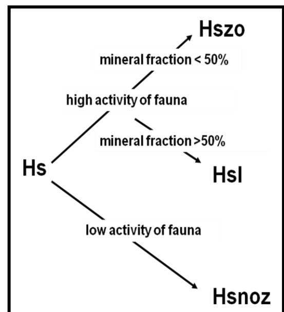
Fig. 19. The different sapric horizons.
