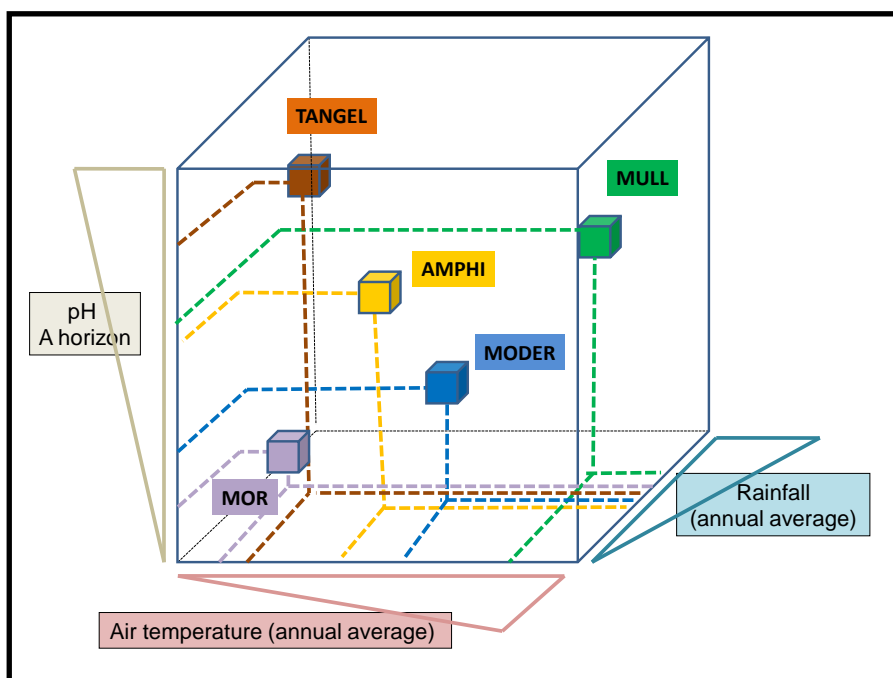
Fig. 13. First attempt at an ecological framework for Terroforms. The gravity centres of the different Terroforms have been positioned in the space of three main factors, temperature, annual rainfall and soil pH, known to influence litter biodegradation. The scheme aims to show the relative position of the main humus forms in a hypothetical three-dimensional space of potential development.
