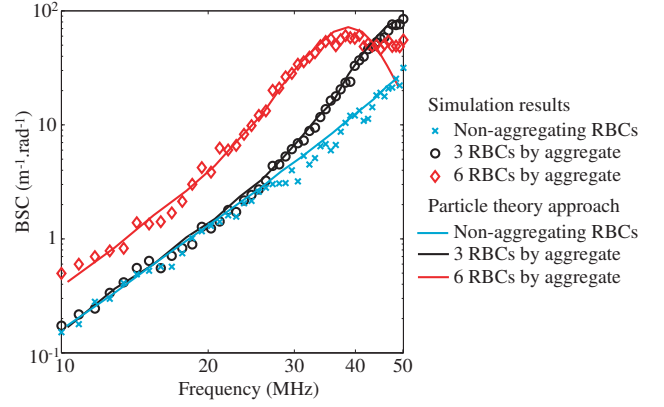
FIGURE 4 – Frequency-dependent backscattering coefficients for a constant hematocrit of 24 % in the case of non-aggregated and aggregated RBCs. The solid line represents the curve for the particle theory approach. Simulations results are shown by the symbols.
