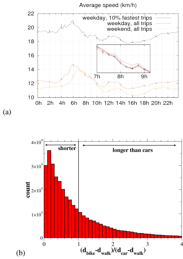
FIG. 2: (a) Average speed vs hour in weekdays and weekends. Bars give the 95% confidence interval. (b) Histogram of (d_{\text{bike}} - d_{\text{walk}}) / (d_{\text{car}} - d_{\text{walk}}) distances for the 375,165 morning (7 to 9am) weekday trips, when bikers are likely to have time constraints.
