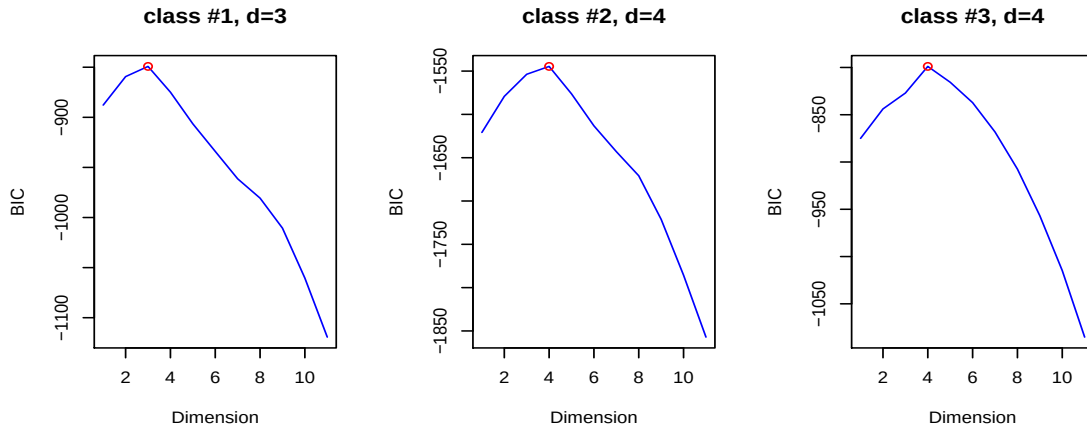
Figure 2: Selection of the intrinsic dimension of the classes in HDDA using the BIC criterion for the wine dataset.
