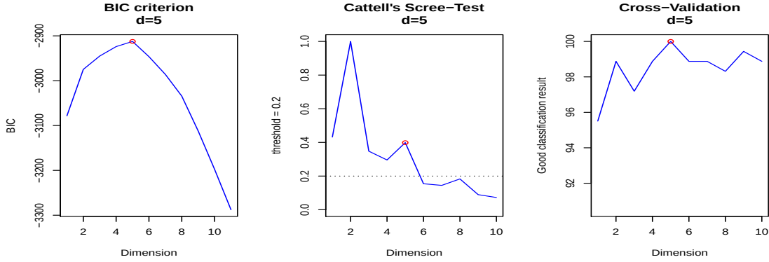
Figure 4: Intrinsic dimension selection with the BIC criterion, Cattell's scree-test and LOO-CV on the wine dataset with the common dimensions model [a_{kj}b_kQ_kd] of HDDA.
