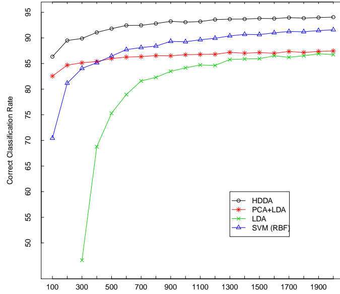
Figure 9: Influence of the size of the learning dataset on prediction results obtained with HDDA and other classification methods on the USPS dataset.
