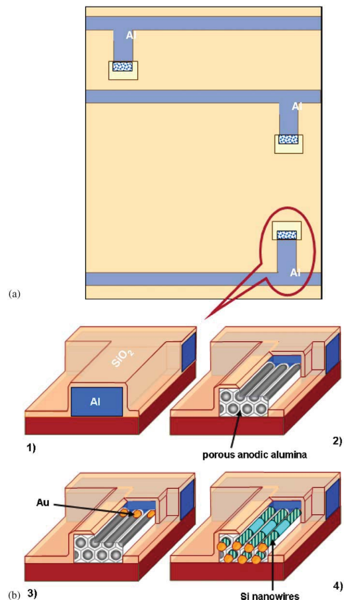
Fig. 4. TFT fabrication in an active matrix: (a) top view of the aluminum lines after deposition and etching followed by \text{SiO}_2 encapsulation and window opening; and (b) the fabrication sequence depicted in Fig. 2 performed in the Al fingers of Fig. 3a.
