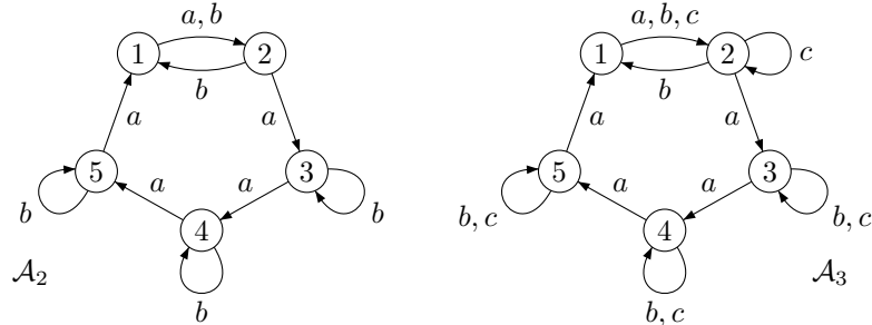
Fig. 1.12. The automata \mathcal{A}_2 and \mathcal{A}_3
