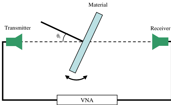
Figure 1: Illustration of the measurement setup
