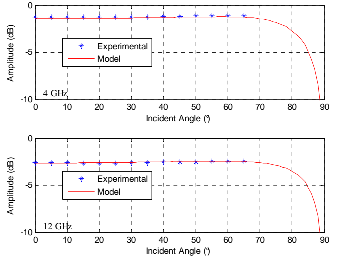
Figure 11: Transmission coefficient of door from measurement and theoretical model using VV polarisation
