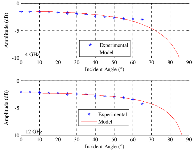
Figure 10: Transmission coefficient of door from measurement and theoretical model using HH polarisation
