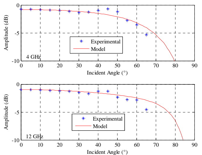
Figure 6: Transmission coefficient of plasterboard from measurement and theoretical model using HH polarisation.
