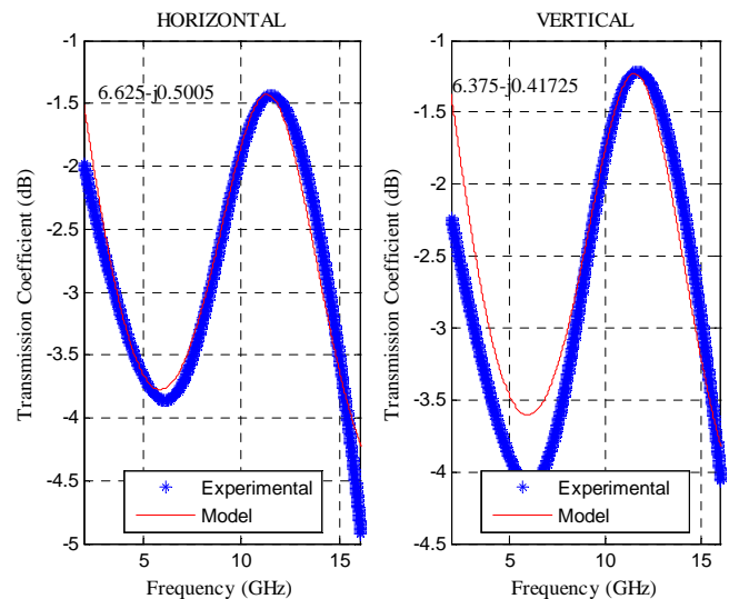
Figure 2: Transmission coefficient of glass from measurement and the theoretical model
