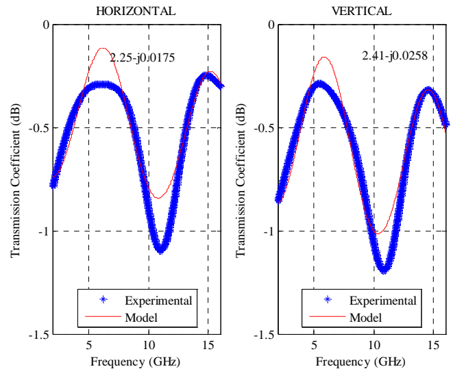
Figure 5: Transmission coefficient of plasterboard from measurement and the theoretical model
