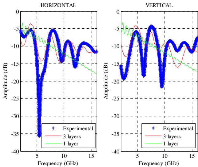
Figure 12: Transmission coefficient of cinder block from measurement and the theoretical model
