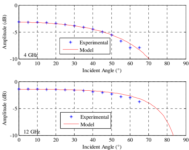
Figure 3: Transmission coefficient of glass from measurement and theoretical model using HH polarisation.
