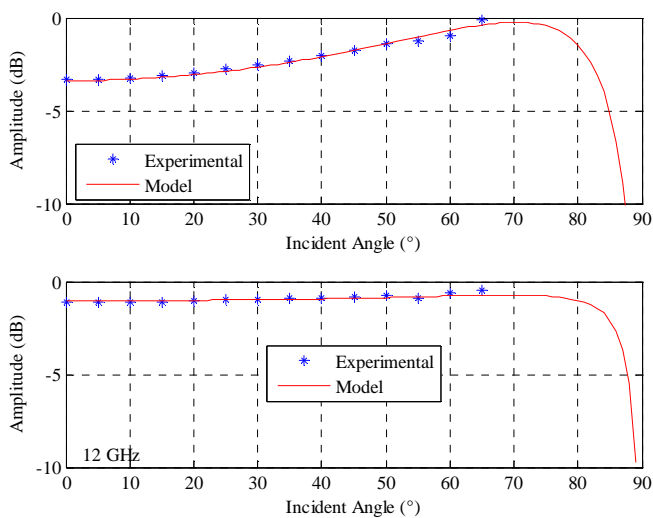
Figure 4: Transmission coefficient of glass from measurement and theoretical model using VV polarisation.
