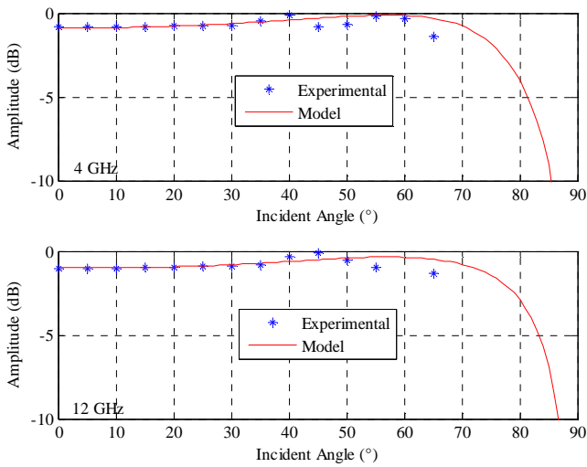
Figure 7: Transmission coefficient of plasterboard from measurement and theoretical model using VV polarisation.
