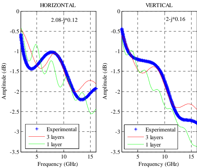
Figure 8: Transmission coefficient of door from measurement and the theoretical model
