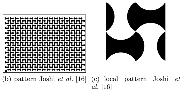
Fig. 5: Calibration patterns for local PSF estimation
