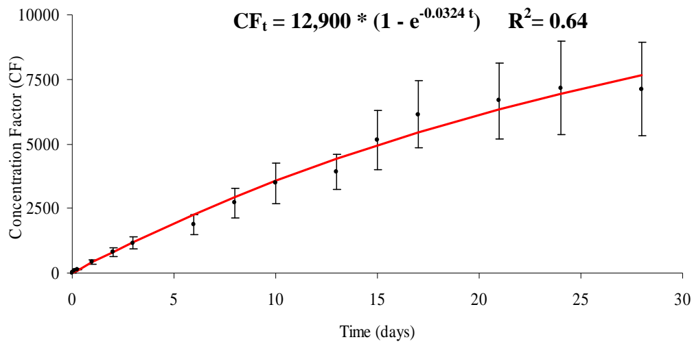
Fig. 1 Uptake kinetics of ^{110m}\text{Ag} in Lobophora variegata (mean concentration factor \pm SD, n = 12)
