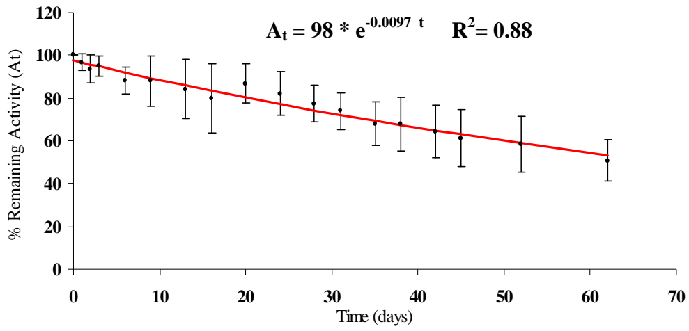
Fig. 2 Depuration kinetics of ^{110m}\text{Ag} in Lobophora variegata (% Remaining Activity \pm SD, n = 12)
