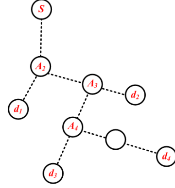
Fig. 2. Demonstration of the worst case of the Member-Only algorithm
