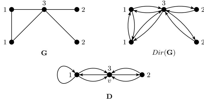
Fig. 1. The labelled digraph Dir(\mathbf{G}) is fibred over the digraph \mathbf{D} . Therefore, Dir(\mathbf{G}) is not minimal. Since Dir(\mathbf{G}) has a unique vertex of degree 3, Dir(\mathbf{G}) is nt -minimal. The digraph \mathbf{D} is minimal and also nt -minimal.
