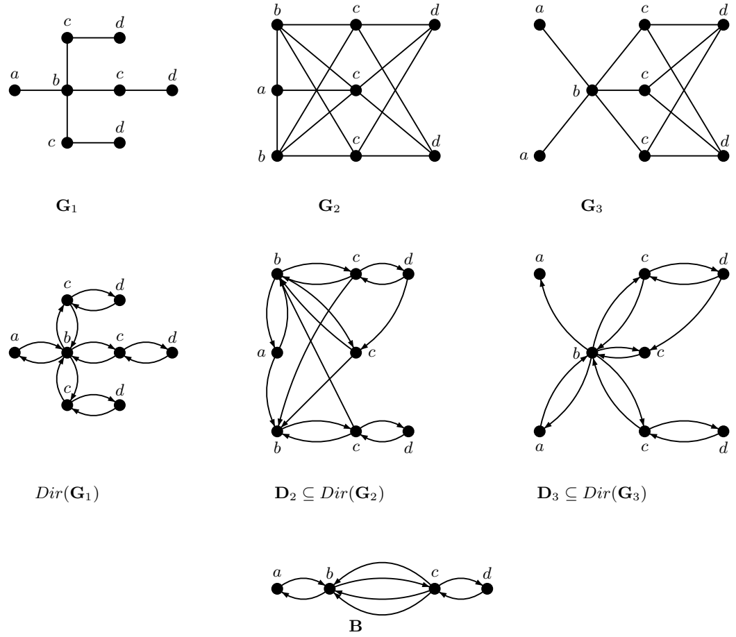
Fig. 2. The labelled digraph Dir(\mathbf{G}_1) is fibred over the digraph \mathbf{B} . This fibration is a t -fibration and Dir(\mathbf{G}_1) is nt -minimal; the subdigraphs \mathbf{D}_2 of Dir(\mathbf{G}_2) and \mathbf{D}_3 of Dir(\mathbf{G}_3) are also t -fibred over the minimal base \mathbf{B} . From Lemma 1, an execution of a leader election algorithm on \mathbf{B} can be lifted to an execution on Dir(\mathbf{G}_1) and an execution on \mathbf{D}_2 and \mathbf{D}_3 . Thus, the vertex a can be declared as elected in \mathbf{B} , \mathbf{G}_1 and \mathbf{G}_2 and the vertex b can be declared as elected in \mathbf{B} , \mathbf{G}_1 and \mathbf{G}_3 . If the algorithm chooses a (resp. b ), then two vertices in \mathbf{G}_2 (resp. \mathbf{G}_3 ) are declared as elected: that is not possible.
