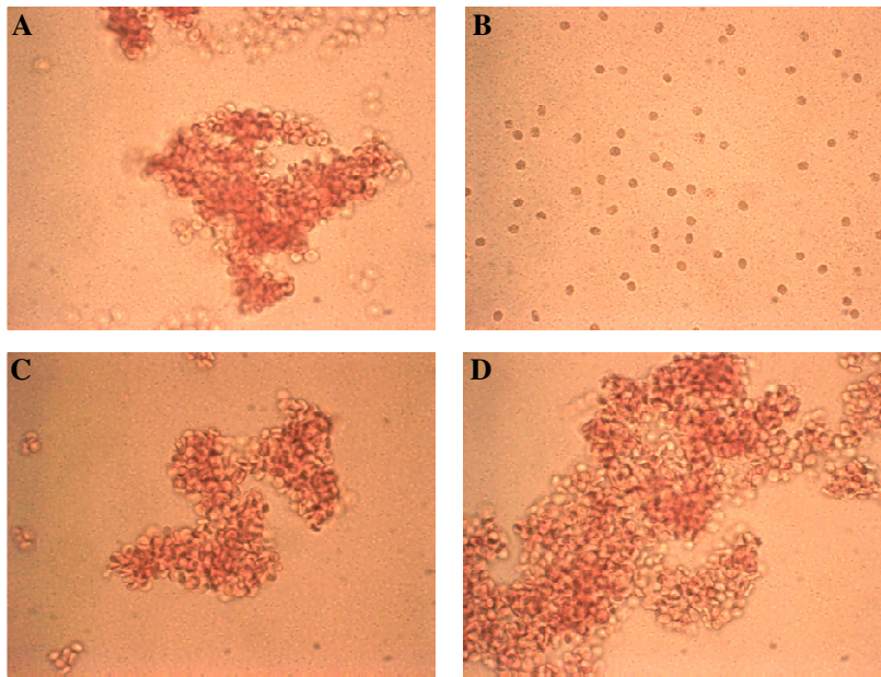
Figure 6 Inhibition assay.
