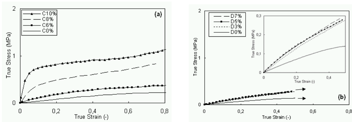
Figure 5: True stress vs. true strain for (a) C-series and (b) D-series Uniaxial tensile test at T_a +50^{\circ}C and \dot{\epsilon} = 0.005s^{-1} using a VideoTraction apparatus [39].
