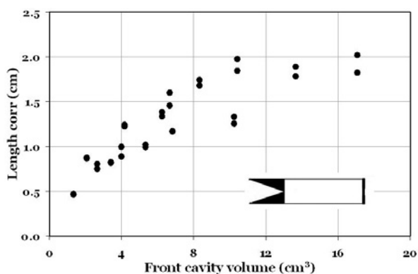
Figure 12. Data pertaining to the study of notched copper tubes. The length corrections for unnotched cylindrical tubes [that generate the formant patterns of the notched tube] are plotted on the y-axis. The volume enclosed by the tube in the notch region is on the x-axis and is illustrated by the blackened 'duck bills' of the tube.
