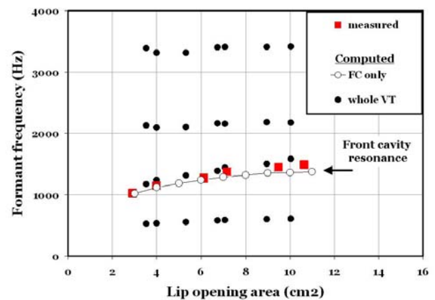
Figure 7. Measured and calculated resonances for the configuration in Figure 5. The diagram shows the effect of lip spreading on the formants of the configuration [red squares] and on values computed on the basis of front cavity volume estimates.
