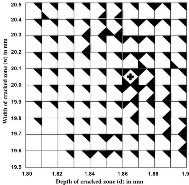
Figure 4: Positions of the elements in matrices of coefficients close to respective target values by 3% - \blacktriangle : A_0 transmission coefficients, \blacktriangledown : S_0 transmission coefficients, \blacktriangleleft : A_0 reflection coefficients, \blacktriangleright : S_0 reflection coefficients, \oplus is the position where all four coefficients are close to the target by less than 3%.
