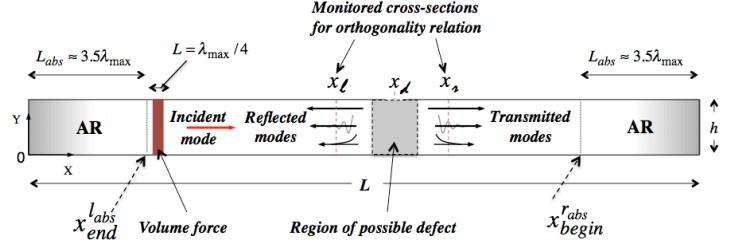
Figure 2: Inverse 2D finite element model.
