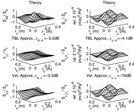
Figure 4: Spatial correlation structures at 275 Hz for the excitation (left) and the panel velocity response (right) due to a TBL (top) and when the TBL (middle) or the velocity are reproduced (bottom) using 3 \times 4 loudspeakers.
