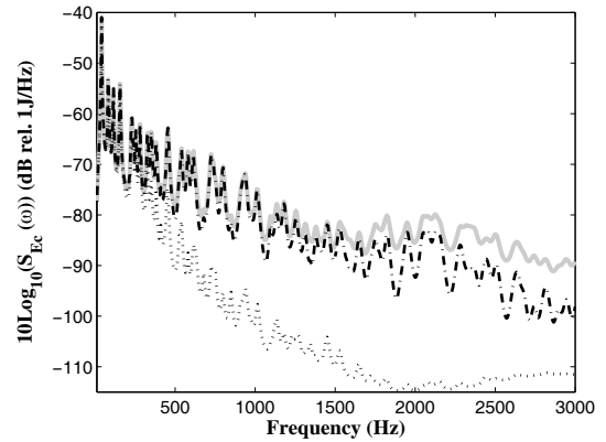
Figure 3 : Panel kinetic energy due to a TBL (grey) and the one generated using a near-field array of 3×4 loudspeakers driven to reproduce the TBL (dotted) or the TBL-induced velocity response (dash-dotted)
