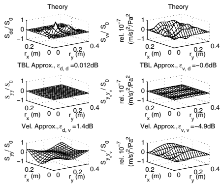
Figure 5: Spatial correlation structures at 634 Hz for the excitation (left) and the panel velocity response (right) due to a TBL (top) and when the TBL (middle) or the velocity are reproduced (bottom) using 3 \times 4 loudspeakers.
