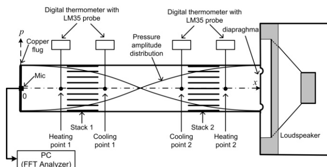
Fig.1 The schematic diagram of the thermoacoustic cooling system with two stacks in a half-wavelength resonator tube.
