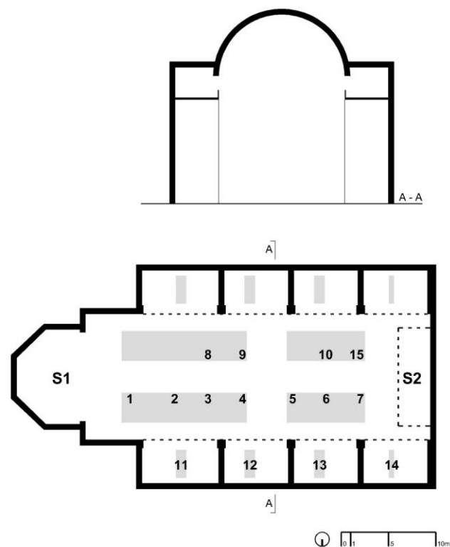
Figure 1: The plan and a section of the Basilica of the Sacred Heart of Jesus
