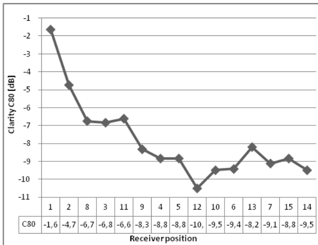
Figure 5: C80 vs. Source S1 – receiver position distance
