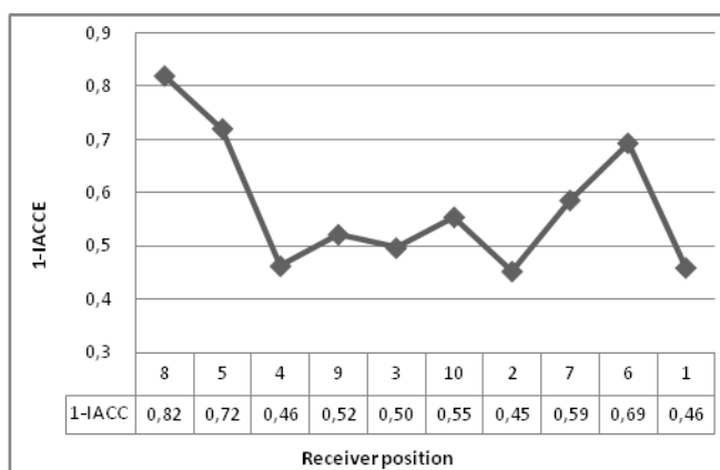
Figure 11: 1-IACC E vs. receiver positions
