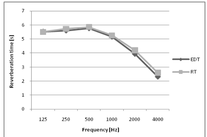
Figure 4: Average Octave Band Reverberation time of the Basilica of the Sacred Heart of Jesus
