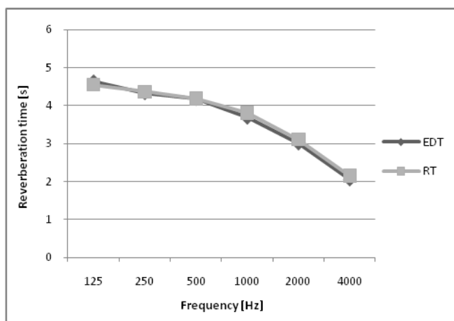
Figure 8: Average Octave Band Reverberation time of the church of the Immaculate Heart of Mary
