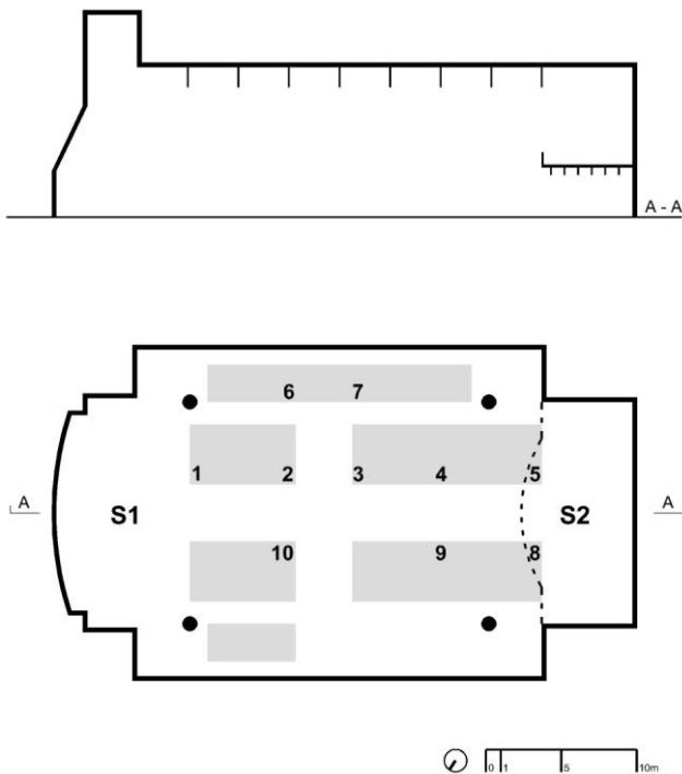
Figure 2: The plan and a section of the church of the Immaculate Heart of Mary
