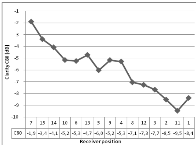
Figure 6: C80 vs. source S2 – receiver position distance
