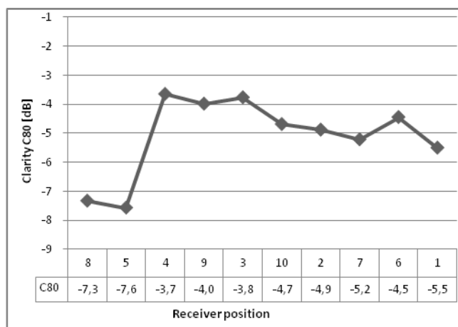
Figure 10: C80 vs. Source S2 – receiver position distance
