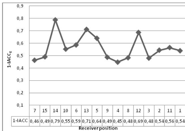
Figure 7: 1-IACC_E vs. Source S2 – receiver distance
