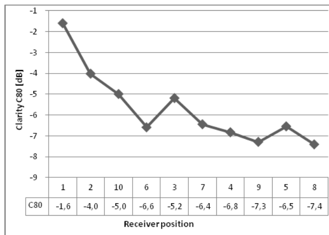
Figure 9: C80 vs. Source S1 – receiver position distance
