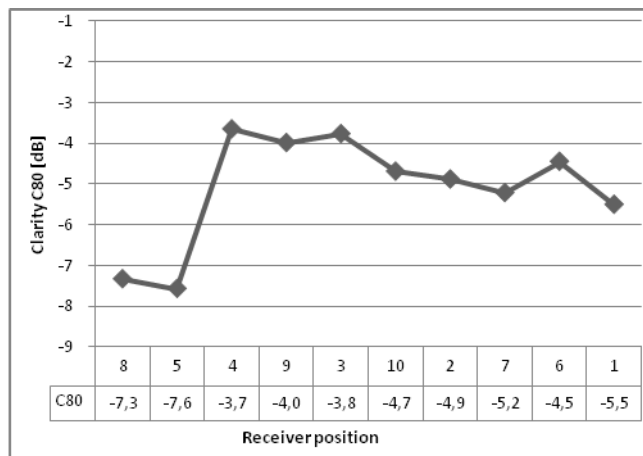
Figure 10: C80 vs. Source S2 – receiver position distance
