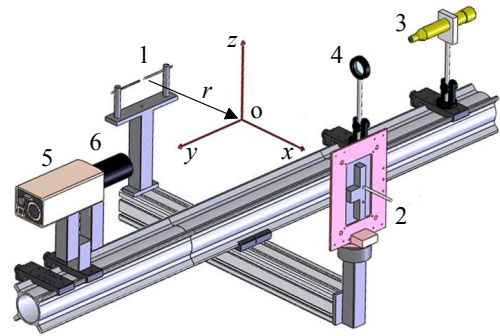
Figure 1: Experimental setup: 1-spark source, 2-microphone in a baffle, 3-Nanolight flash lamp, 4-focusing lens, 5-camera, 6-lens.
