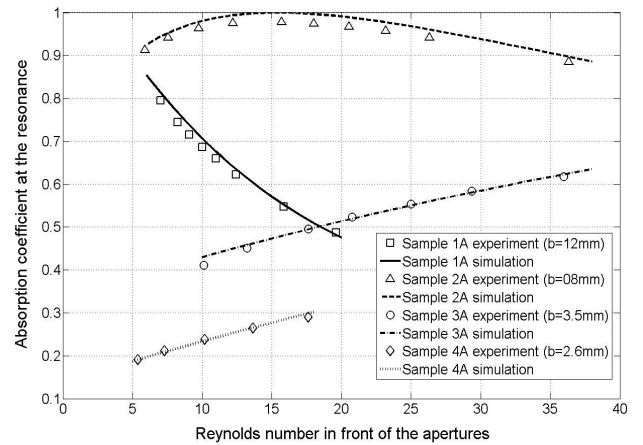
FIG. 6 – Absorption coefficient at the resonance as a function of the Reynolds number in front of the apertures for group A samples. Excitation frequency of 506 Hz.
